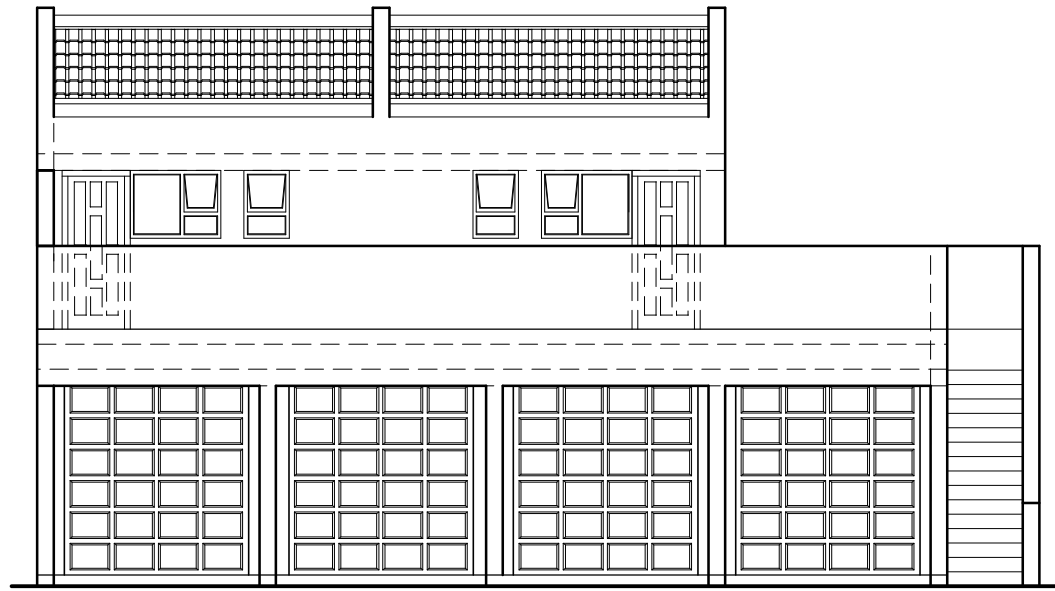
FRONT ELEVATION
